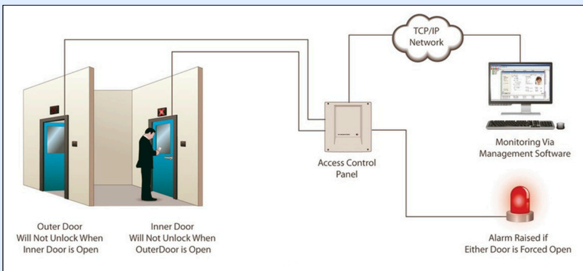
Door Interlocking & Access Control System
