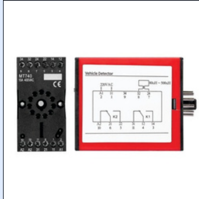
Metal Loop Detector
