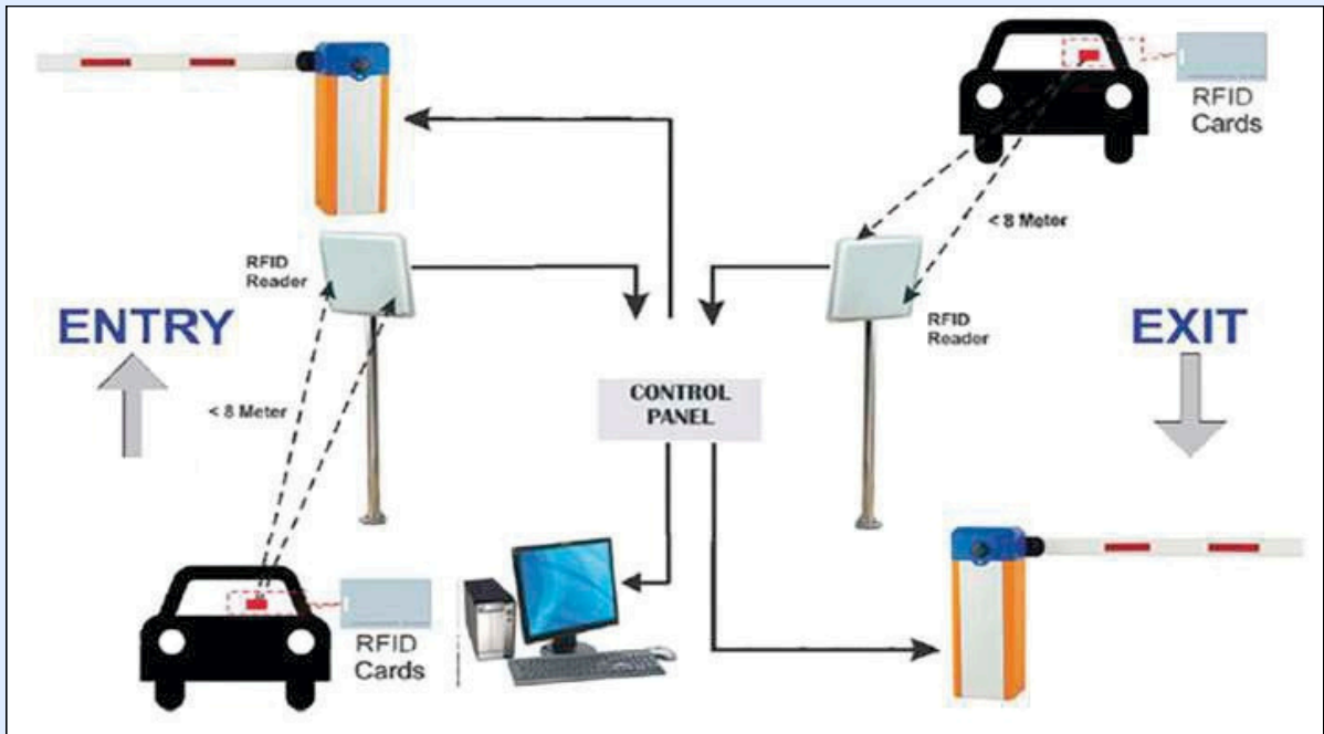
Automatic Number Plate Reading System (ANPR)
